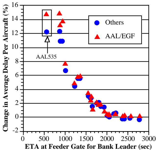
Figure 3 Change in average delays per aircraft when priority scheduling is used instead of FCFS scheduling
