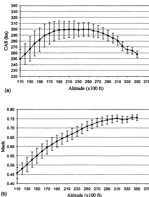
Fig. 5 Mean MD-80 climb profiles for 249 aircraft recorded November 1999: (a) CAS, (b) Mach.
