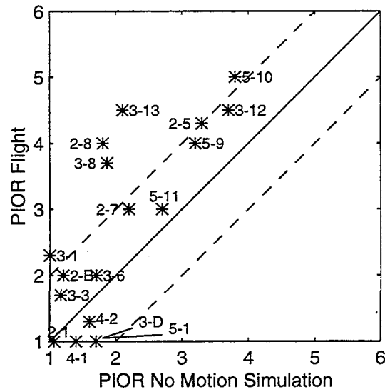
Figure 16 – Flight versus no motion PIORs
