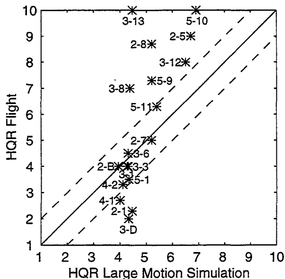
Figure 10 – Flight versus large motion HQRs
