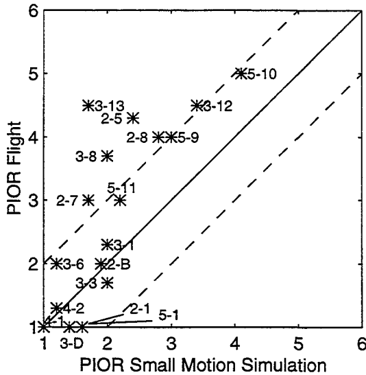
Figure 15 – Flight versus small motion PIORs
