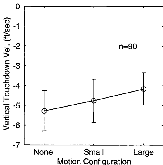
Figure 8 – Touchdown velocities
