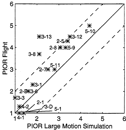
Figure 14 – Flight versus large motion PIORs
