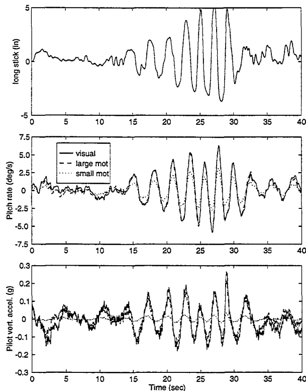
Figure 7 – Example PIO
