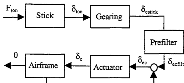
Figure 2 – Longitudinal block diagram
