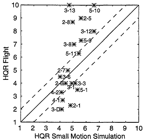
Figure 11 – Flight versus small motion HQRs
