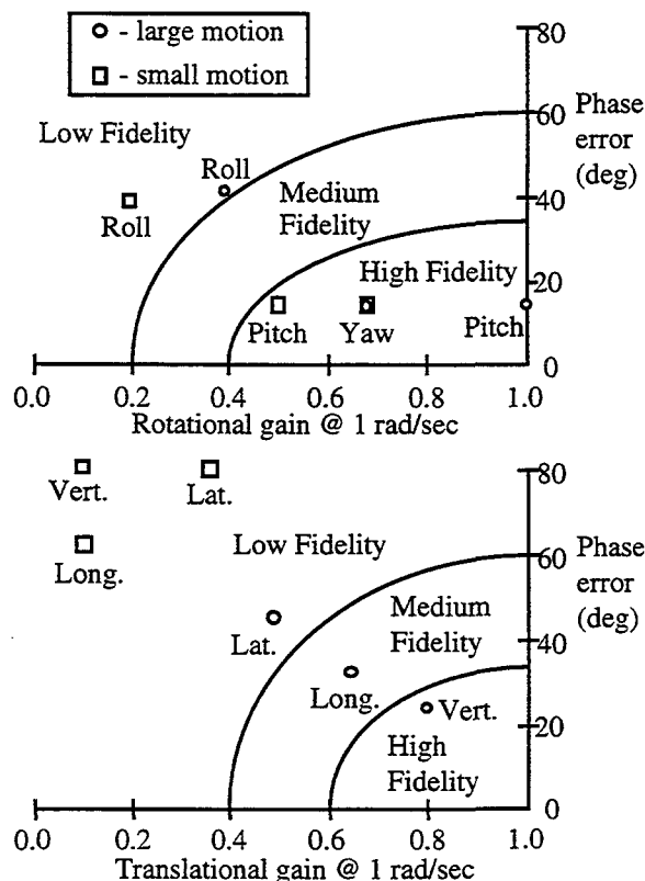
Figure 6 – Motion fidelity prediction
