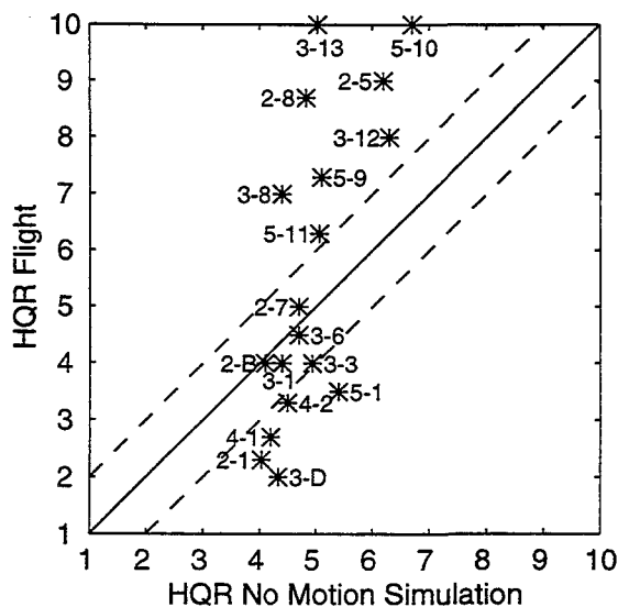
Figure 12 – Flight versus no motion HQRs
