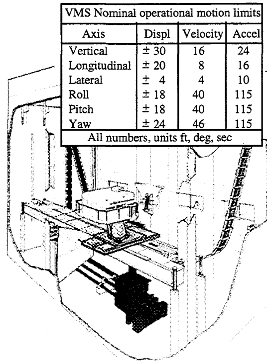
Figure 3 – NASA Ames Vertical Motion Simulator
