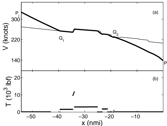
Figure 5. The minimum-cost speed profile and control strategy for the Min-Fuel condition.
