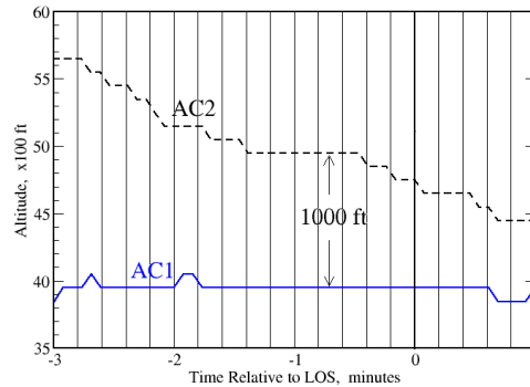
Figure 13. Altitude profiles for a sample late-detection operational error.
