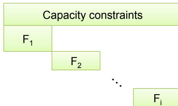
Figure 1. The block-angular form of the Bertsimas-Stock Patterson model. Each F_i represents the complete physical and temporal constraints of a distinct set of flights.
