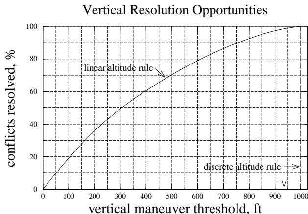
Figure 13: Vertical resolution opportunities: percentage of conflicts resolved as a function of vertical maneuver threshold
