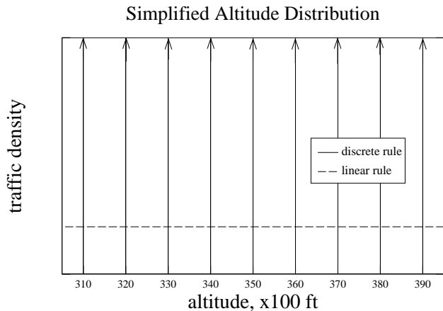
Figure 2: Simplified altitude distribution for enroute traffic in a representative altitude range, for the discrete and linear altitude rules
