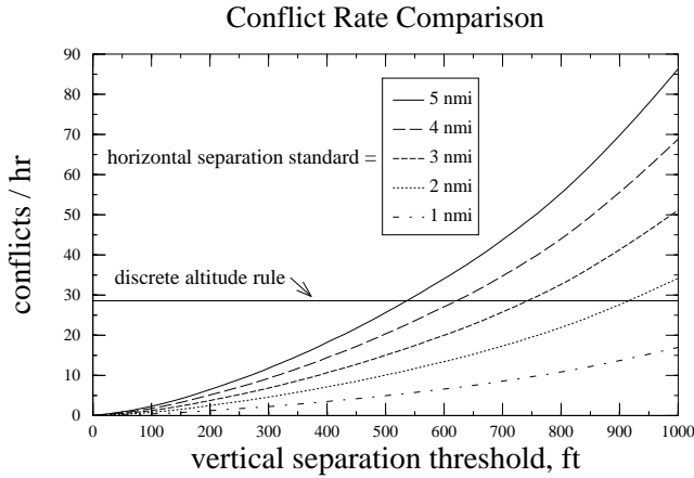
Figure 12: Conflict rate as a function of vertical separation threshold for the linear altitude rule, with horizontal separation standard as a parameter
