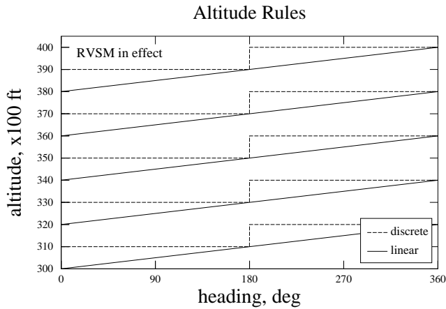
Figure 1: Designated altitude as a function of heading (or course) for level flight in a representative altitude range, for the discrete and linear altitude rules
