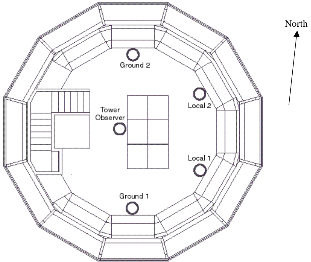
Figure 4: FFC Controller-Position Diagram
