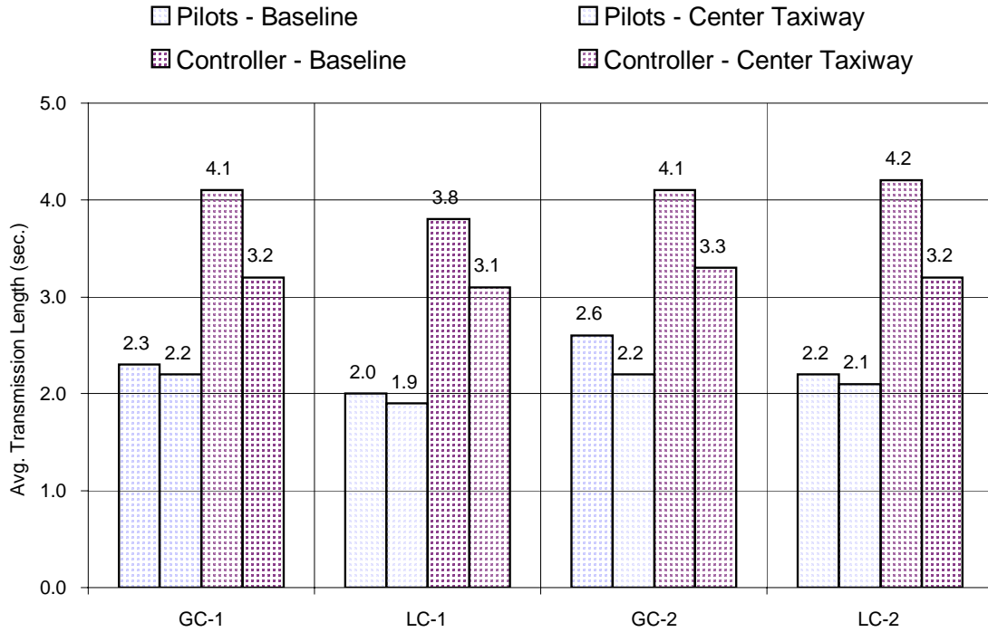
Figure 8: Average Transmission Length (sec)
